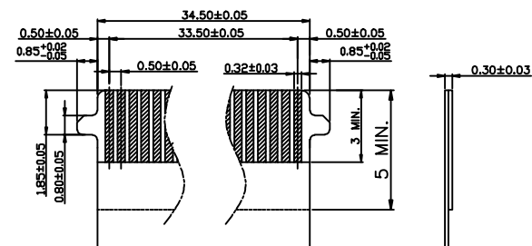
RECOMMENDED FFC DIM. WITH LOCK
