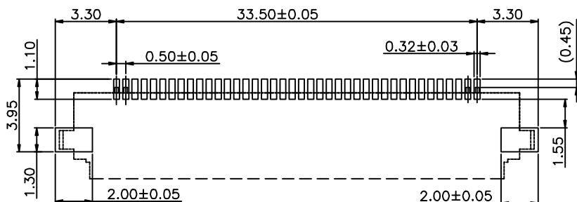
P.C.B LAYOUT REF TOLERANCE:±0.05
